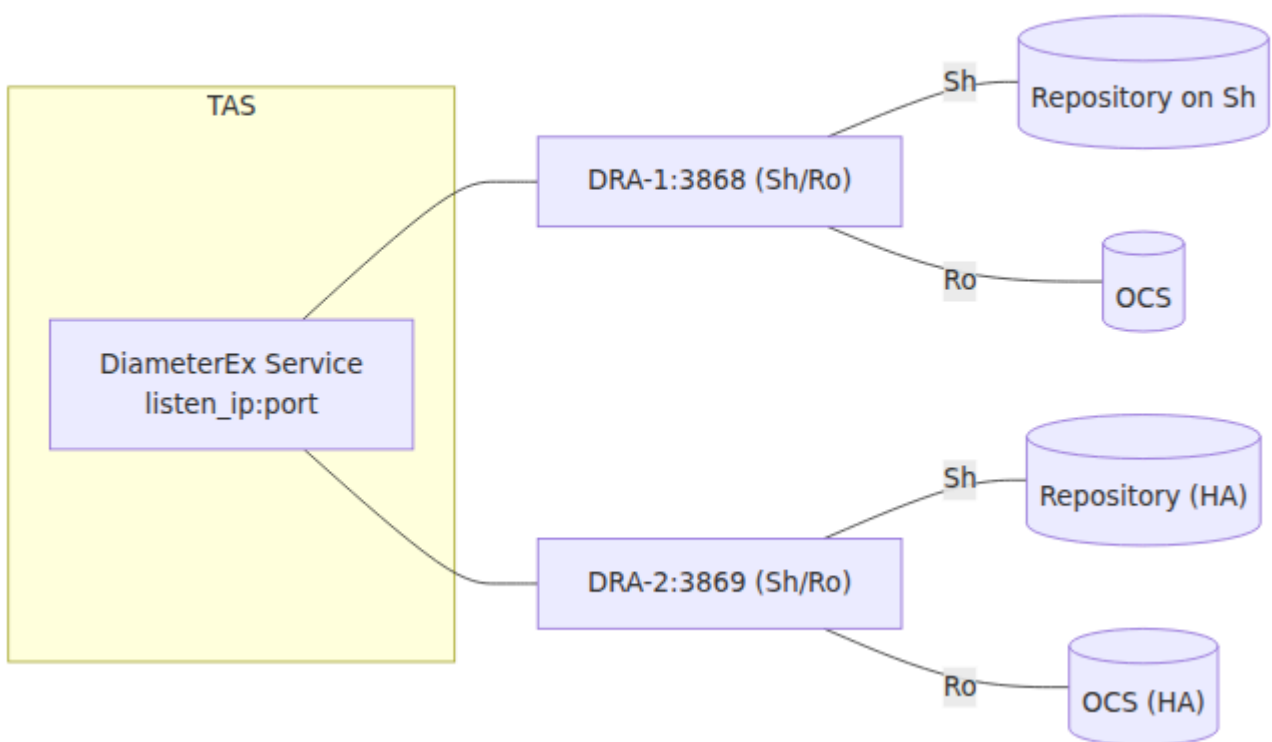
Diameter Peer Connectivity
